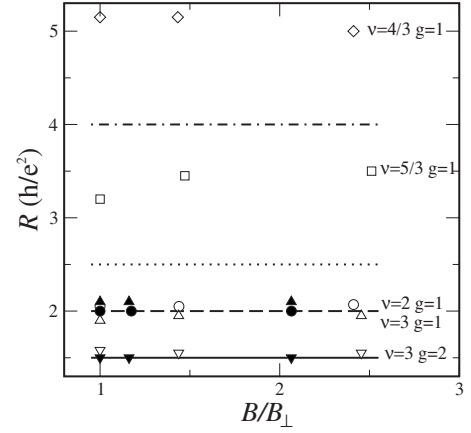
FIG. 5. Slopes R of the linear positive branch of the experimental I - V s for different filling factor combinations as a function of the total magnetic field. Open symbols are for the wafer A: \nu=3, g=2 (down triangles, normal field is B_{\perp}=2.38 T), \nu=3, g=1 (up triangles, B_{\perp}=2.38 T), \nu=2, g=1 (circles, B_{\perp}=3.58 T), \nu=5/3, g=1 (squares, B_{\perp}=4.29 T), \nu=4/3, g=1 (diamonds, B_{\perp}=5.36 T). Filled symbols are for the corresponding \nu and g for wafer B ( B_{\perp}=5.18 T for \nu=3 , 7.69 T for \nu=2 ). Lines indicate the equilibrium slopes R_{eq} : solid line is for \nu=3, g=2 , dash is for \nu=2, g=1 and \nu=3, g=1 , dotted one is for \nu=5/3, g=1 , dash-dot is for \nu=4/3, g=1 .
