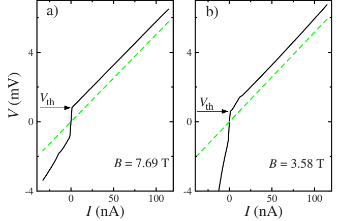
FIG. 3. (Color online) Examples of I - V curves (solid) for the filling factor combinations \nu=2, g=1 for samples with different electron concentrations [(a) and (b) are for wafers B and A, correspondingly]. Calculated equilibrium I - V 's are shown by the dashed lines ( R_{eq} = 2h/e^2 ). The positive branch ( V > V_{th} ) of the experimental curve is linear and parallel to the equilibrium line in both cases. The threshold voltage V_{th} is also denoted. Normal magnetic fields equal to (a) 7.69 T and (b) 3.58 T.
